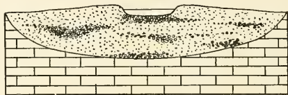
FIG. 10. Diagram showing general structure of stream deposits.
